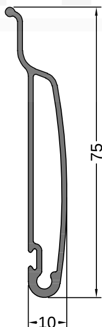
14441 0.555 Kg/m CORTINA TABLILLA REGULABLE
