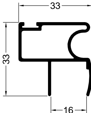
12900 0.459 Kg/m HOJA JAMBA 16 mm.
