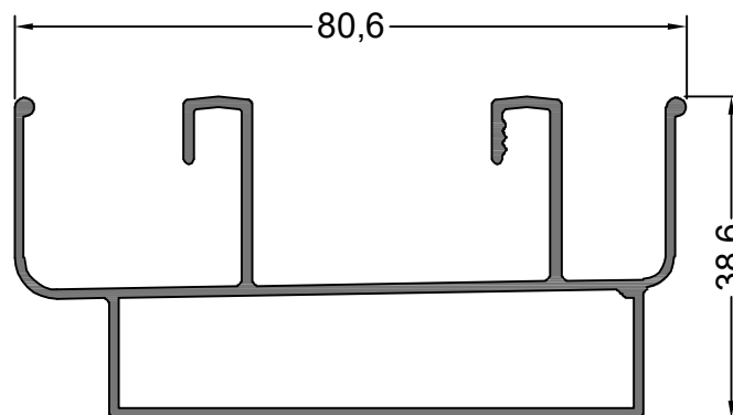
13420 0.935 Kg/m CORREDIZA MARCO UMBRAL
