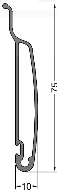
14441 0.555 Kg/m CORTINA TABLILLA REGULABLE
