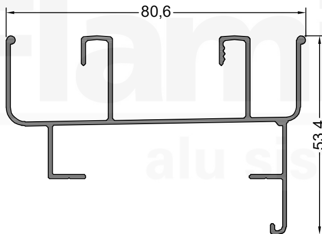
13491 0.793 Kg/m CORREDIZA MARCO JAMBA Y DINTEL
