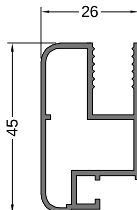
12690 0.582 Kg/m CORREDIZA MOSQUITERO HOJA
