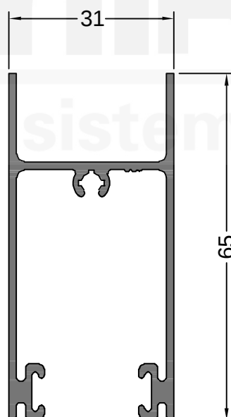
12137 0.806 Kg/m
